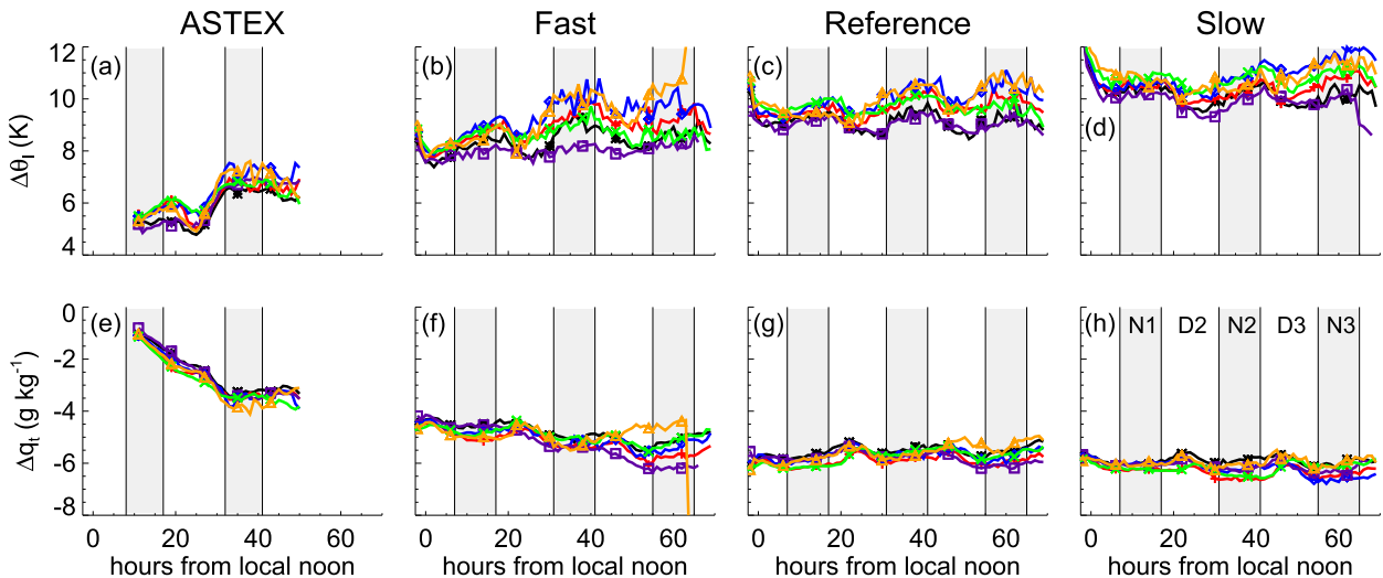
FIG. 11. Time evolution of the inversion jumps of (a)–(d) \Delta\theta_t and (e)–(h) \Delta q_t . The gray shaded bands indicate nighttime periods according to Table 3. The line colors and symbols are as in the legend in Fig. 4a.
