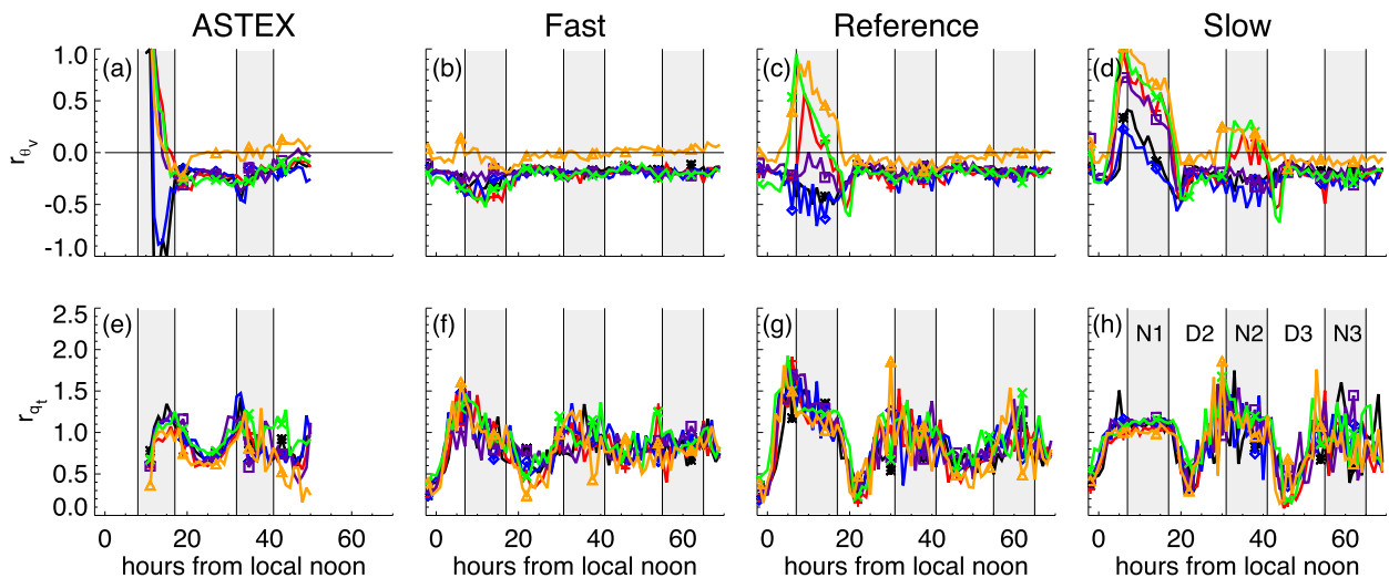
FIG. 10. The time evolution of the flux ratios for the (a)–(d) buoyancy r_{\theta_v} and (e)–(h) the total water specific humidity r_{q_t} , computed according to Eq. (2). The line styles are according to the legend. The gray shaded bands indicate nighttime periods according to Table 3. The line colors and symbols are as in the legend in Fig. 4a. The thin solid black horizontal line in (a)–(d) represents the zero line.
